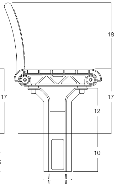
Y-Base Embedded
